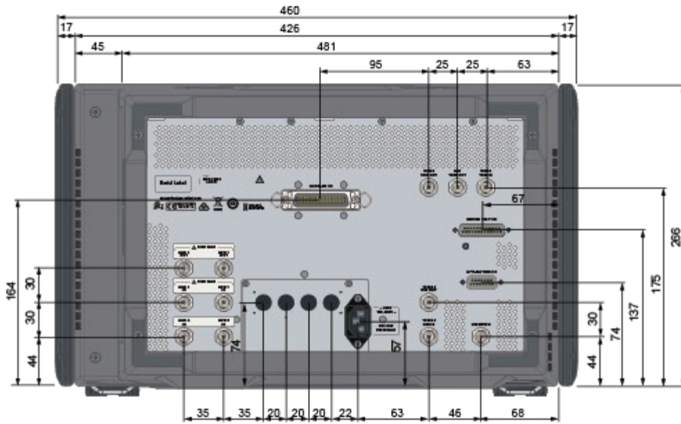
Dimensions (rear view, E5080B with option 1E5/175, in millimeters)
